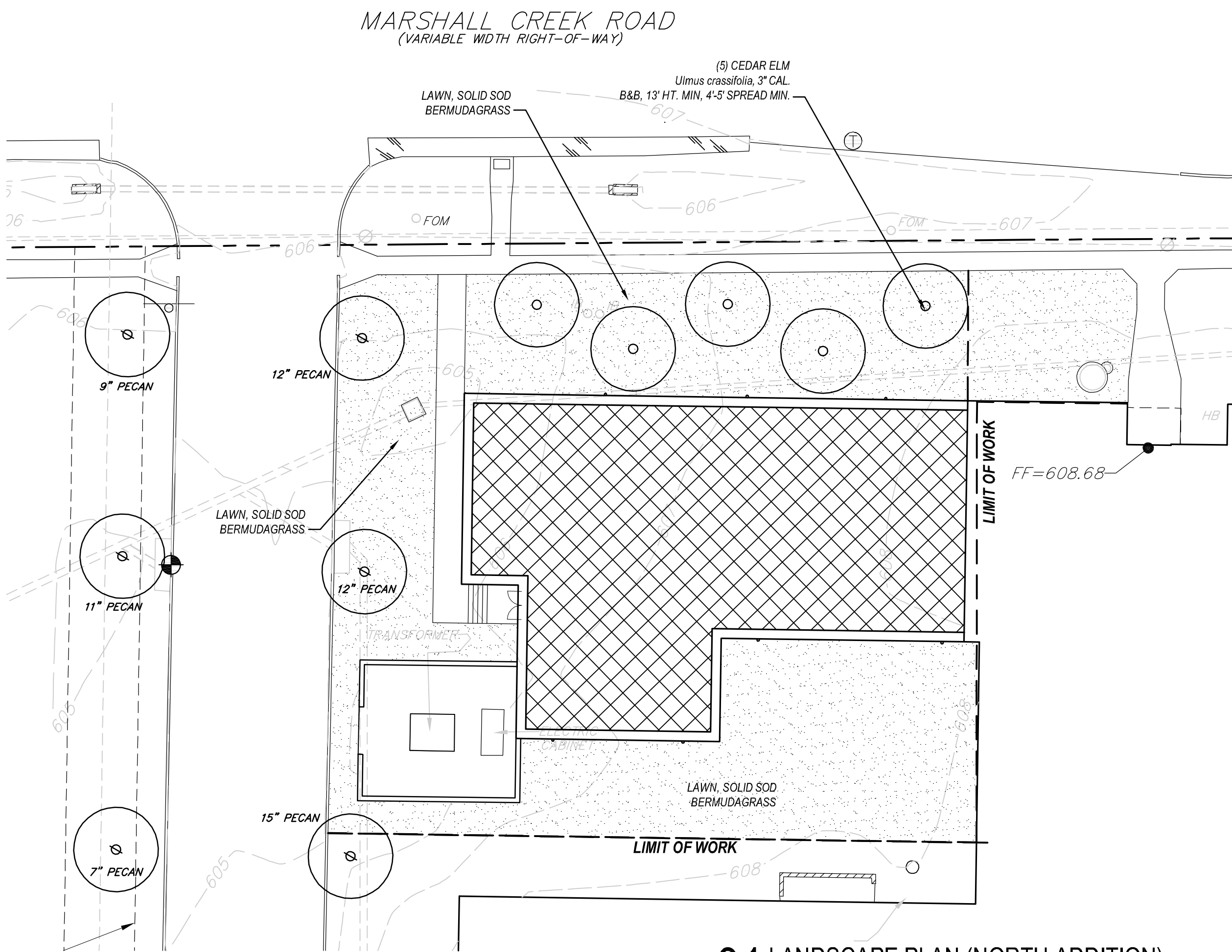
01 LANDSCAPE PLAN (NORTH ADDITION)
