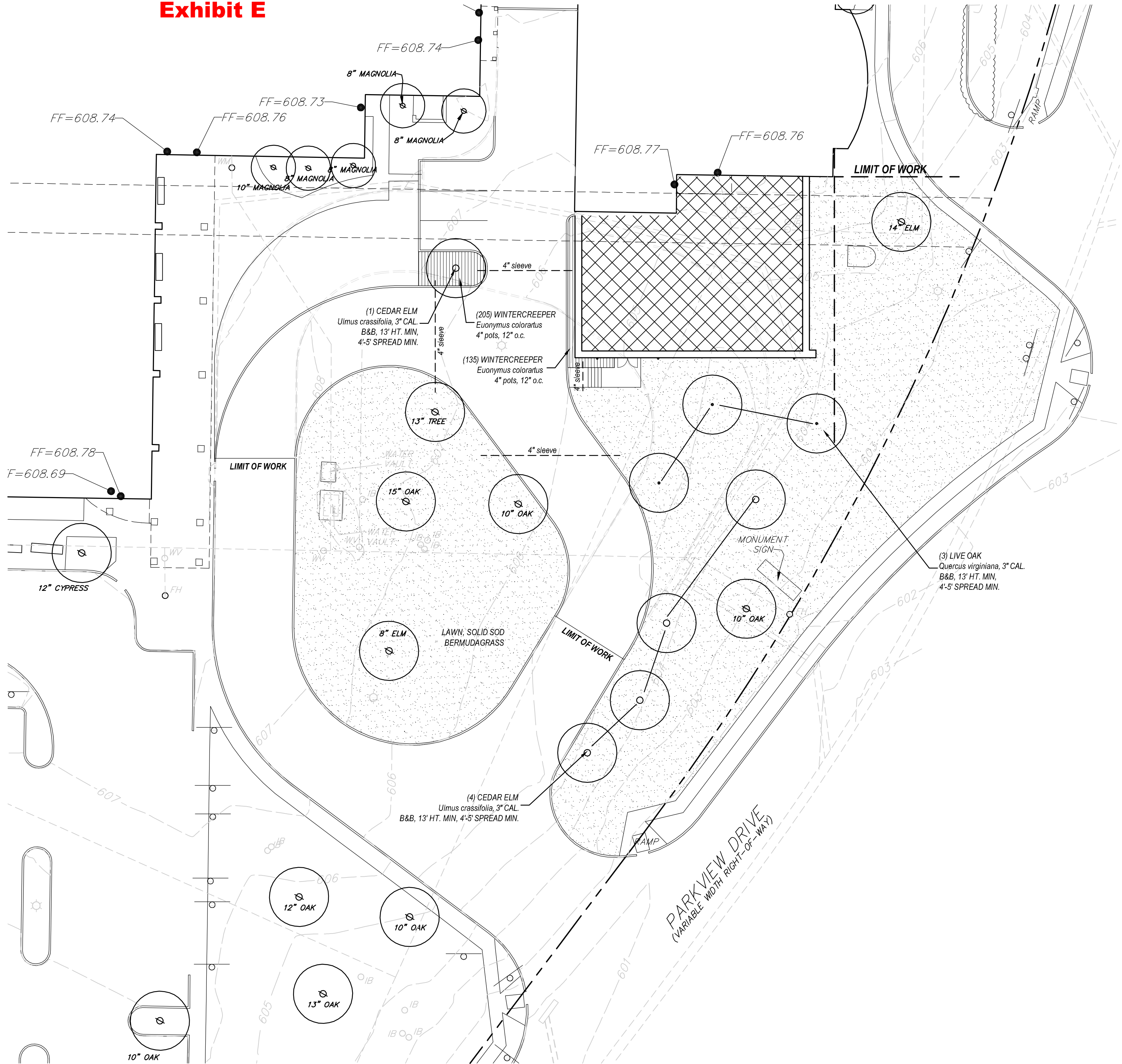
02 LANDSCAPE PLAN (SOUTH ADDITION)
